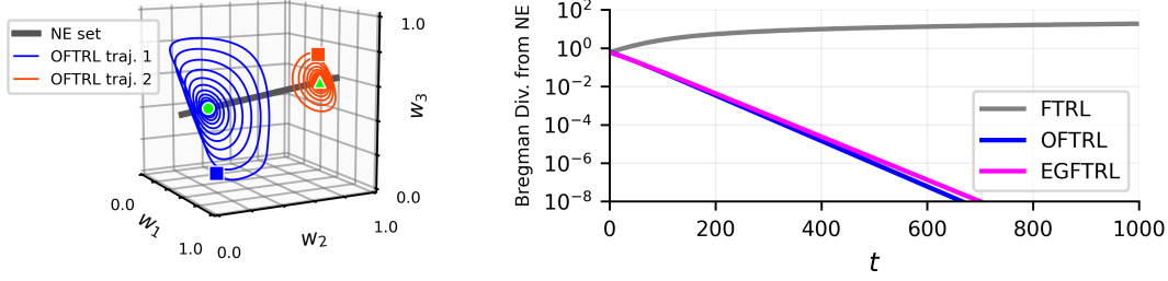
Figure 1: Variants of FTRL (with entropy regularizer) on the 3-player harmonic game in A.4.1. Left: two trajectories of OFTRL converging to their distinct analytic limits (in green) from Theorem 4.1 (i). Right: Bregman divergence from NE for the t -th iterate of OFTRL, EGFTL, and FTRL from a fixed initialization. OFTRL and EGFTL converge linearly (Theorem 4.1(ii)), while FTRL diverges at a geometric rate (Theorem 4.5).
