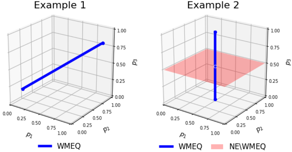
Figure 2: The sets \text{WMEQ}_M(G) and \text{NE}(G) \setminus \text{WMEQ}_M(G) for the instantiation of Example 1 from Section A.4.1 with m_1 = 3, m_2 = 6, m_3 = 4 (left), and Example 2 from Section A.4.2.
